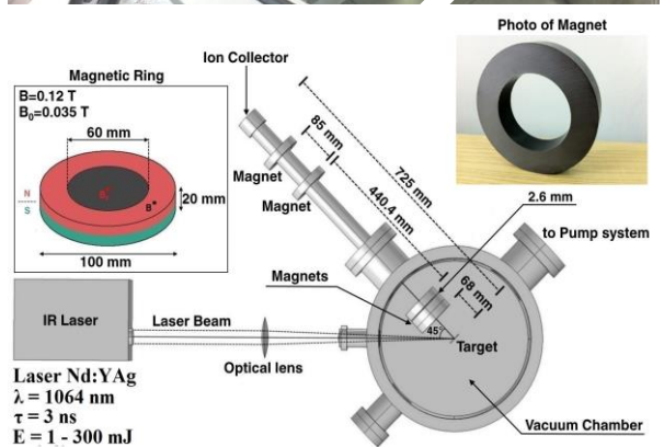
Figure 1: Photo and Scheme of experimental setup.
